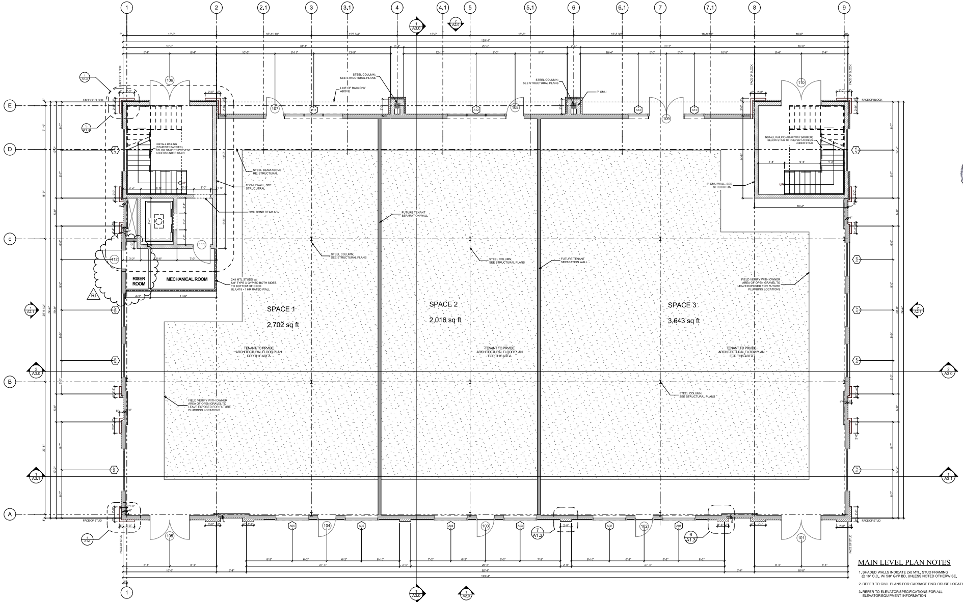
FIRST LEVEL FLOOR PLAN SCALE: 3/16" = 1'-0" ①
